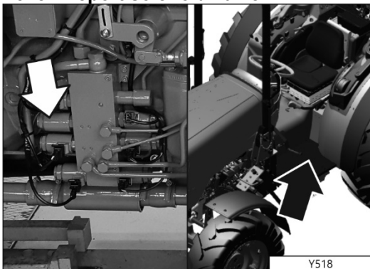
Y518 - Deport solenoid valve 4
