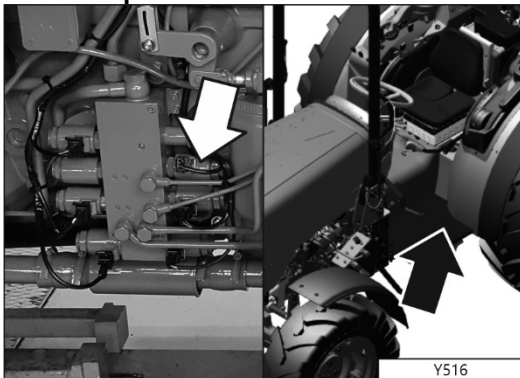
Y516 - Deport solenoid valve 5
