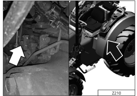
Z210 - DIR PTO selector switch
