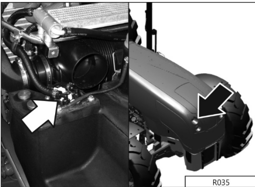
R035 - Fuel level sensor
