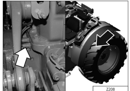
Z208 - 540E/1000 PTO speed selector switch
