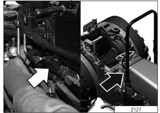
Z127 - RHS brake pedal switch
