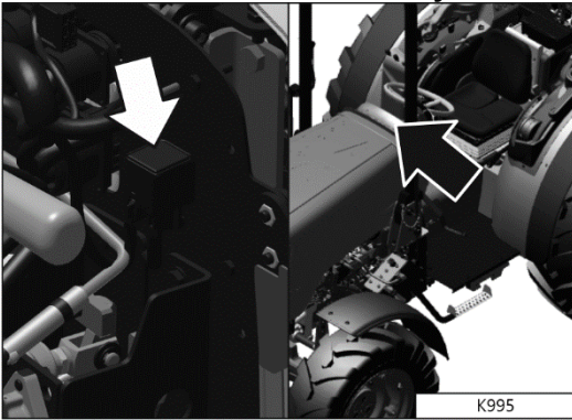
K995 - Front PTO interlock relay
