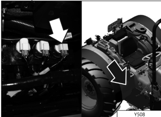
Y508 - FL solenoid valve (Power Reverse Version)
