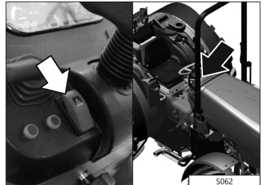
S062 - Hazard switch
