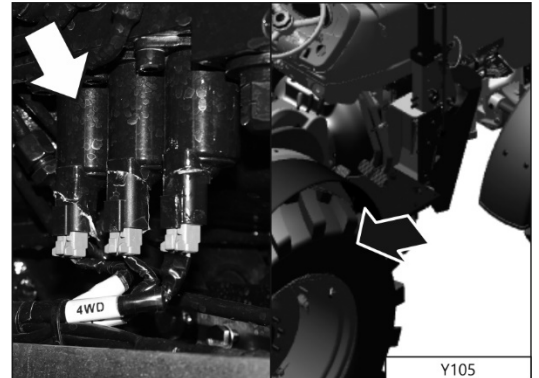
Y105 - Diff-lock solenoid valve
