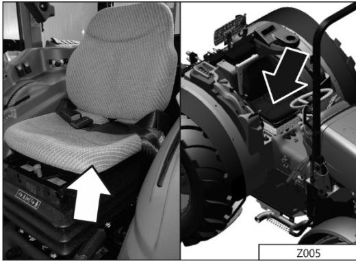
Z005 - Seat switch
