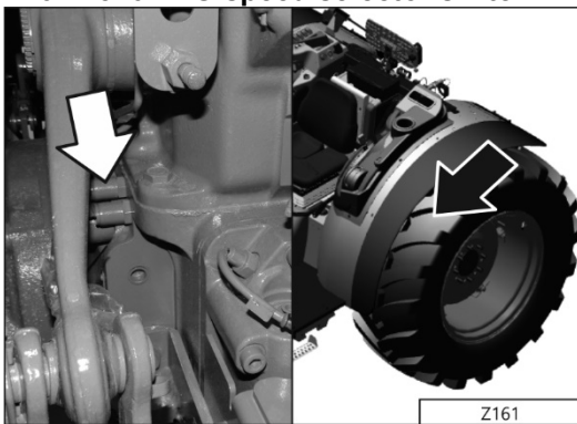
Z161 - 540 PTO speed selector switch
