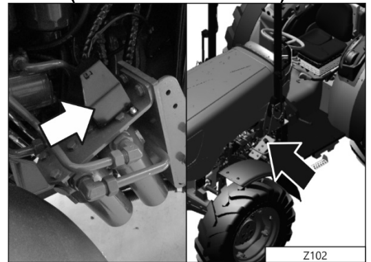
Z102 - Transmission oil filter clogged switch (Power Reverse Version)
